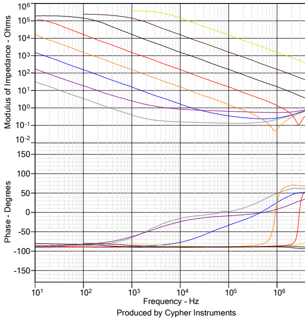
Capacitors
