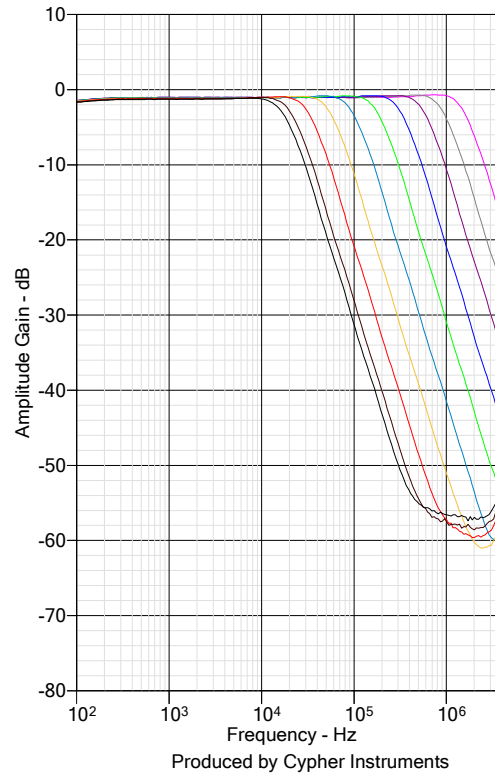
Voltage controlled filter LP 19KHz - 1.5MHz
