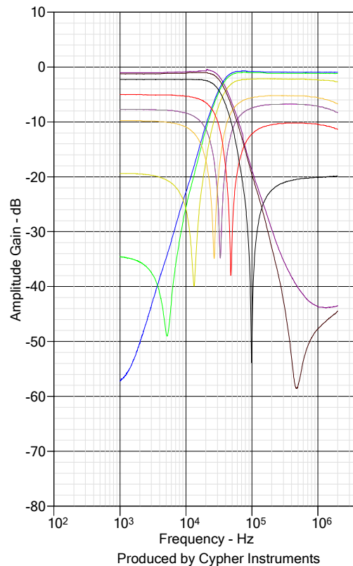
Voltage controlled filter notch 19KHz - 1.5MHz
