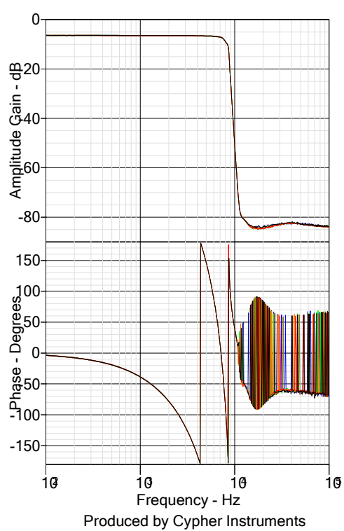
8KHz LC filter module circa 1980
