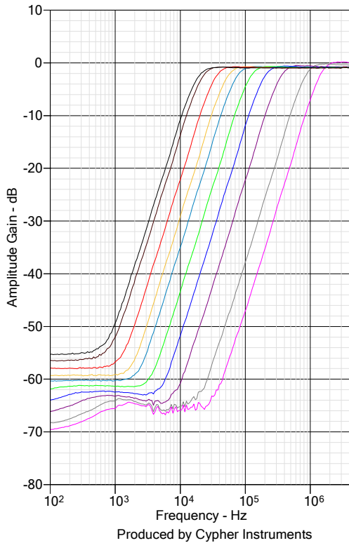
Voltage controlled filter HP 19KHz - 1.5MHz
