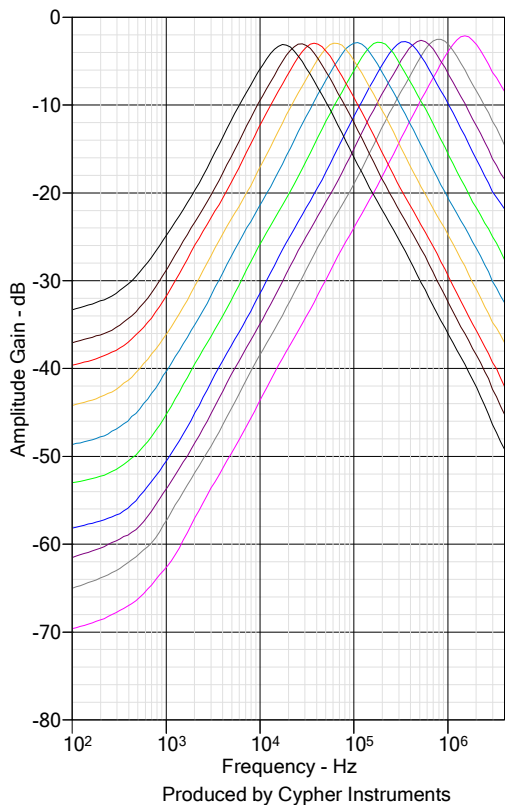
Voltage controlled filter BP 19KHz - 1.5MHz
