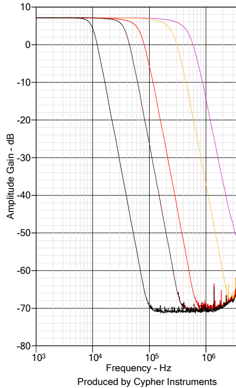
8KHz LC filter module circa 1980
