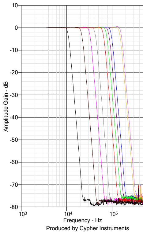
Low pass 8th order
