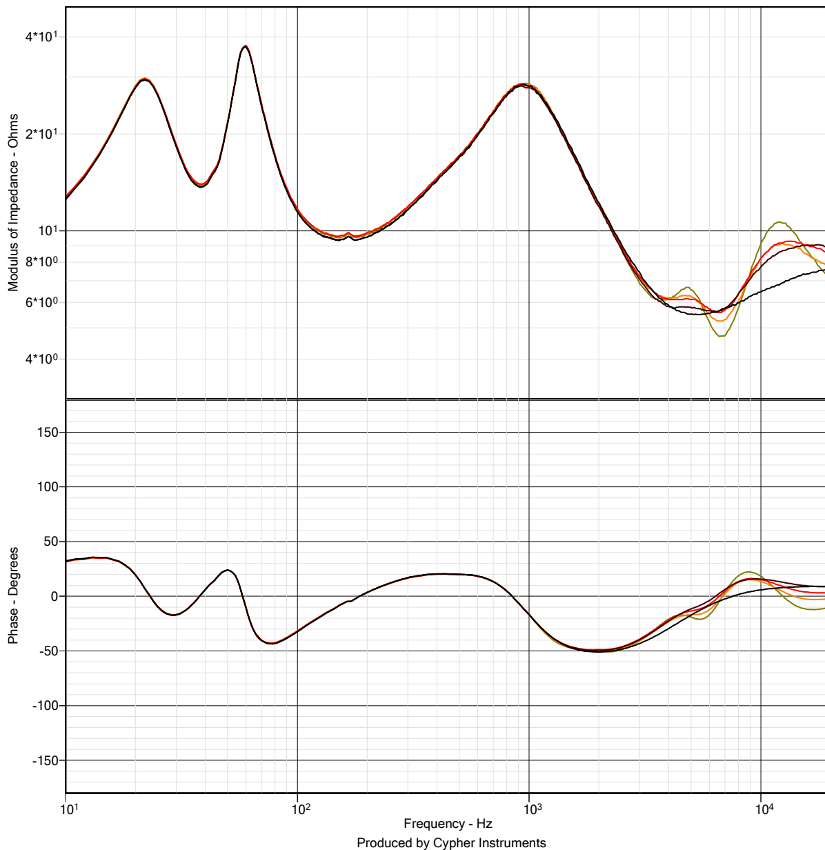
Figure 2. Impedance of a loud speaker
