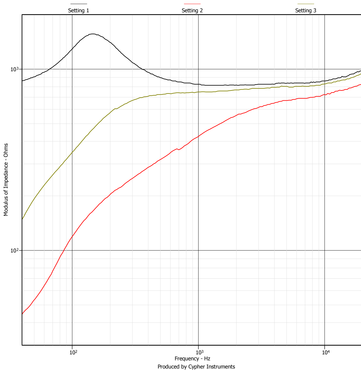
Figure 2. Impedance response of a microphone
