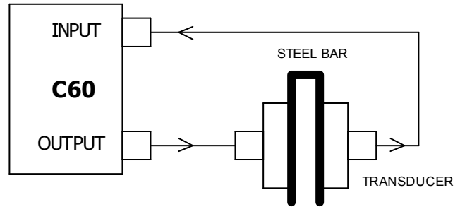
Figure 1. Connection diagram
