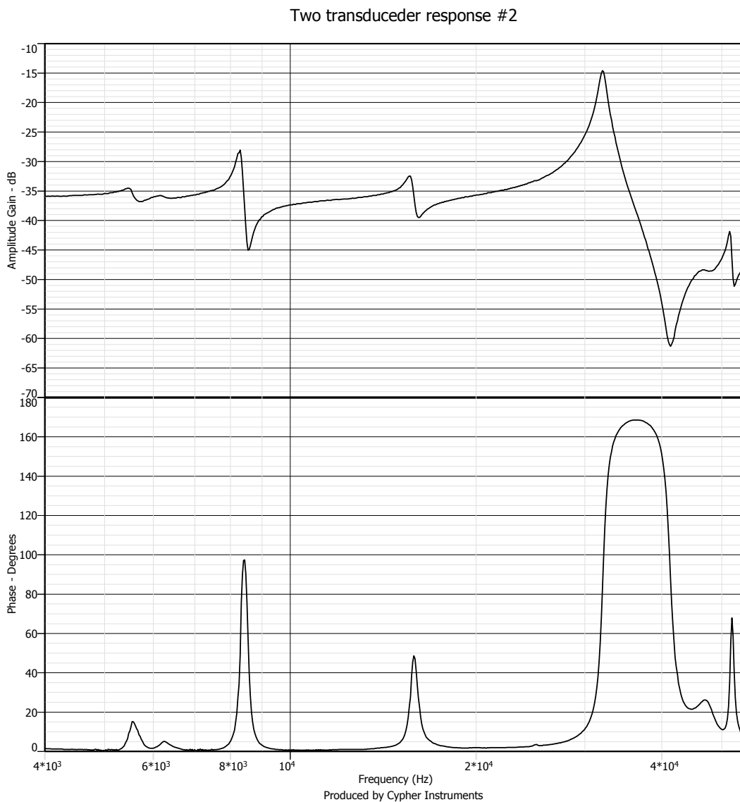
Figure 2. Amplitude response of acoustically coupled system
