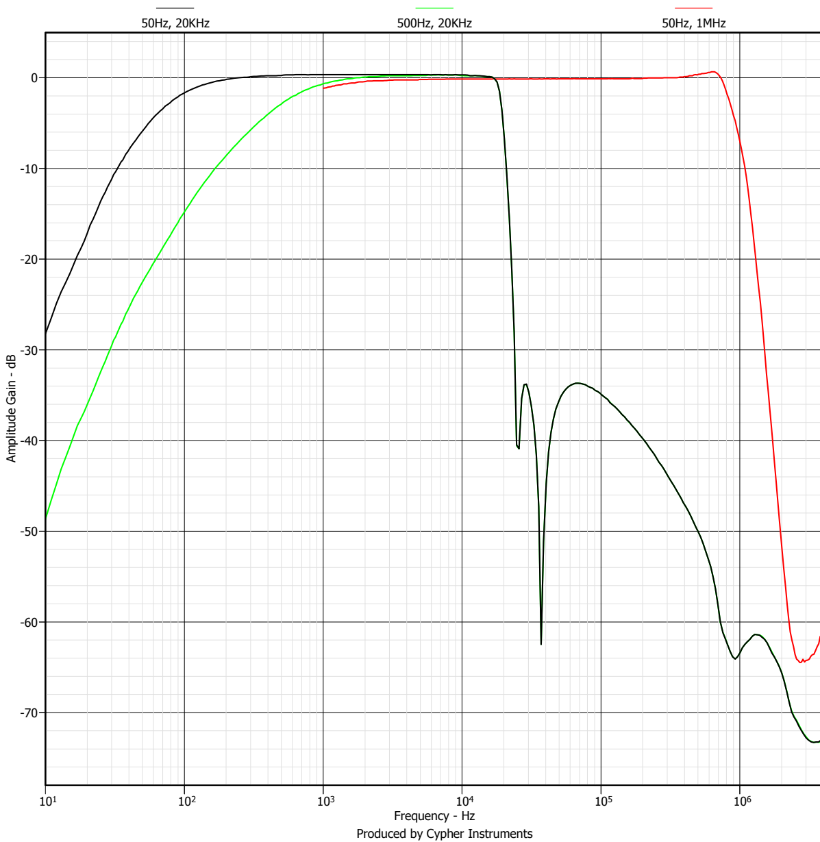
Figure 1. Low noise laboratory preamplifier
